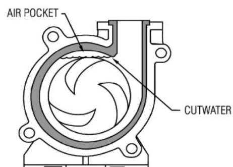
ZERO° STANDARD VERTICAL DISCHARGE CONFIGURATION
