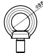
Lifting Eyebolt M16 Z=4
