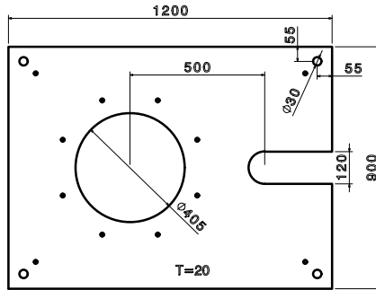
Housing Bearing Support.
